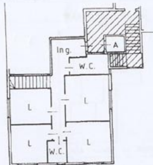
PIANO QUINTO h = 3.00
